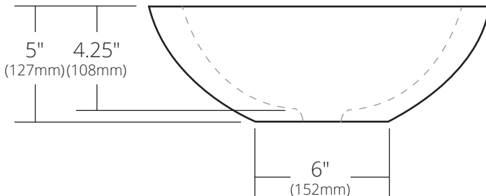
SIDE VIEW
