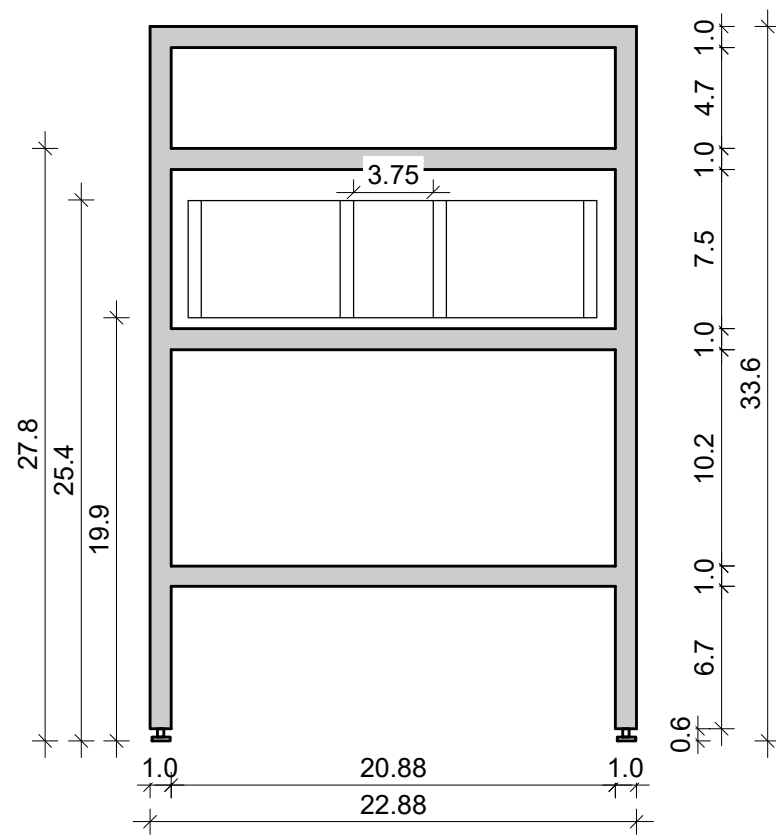
BACK VIEW
