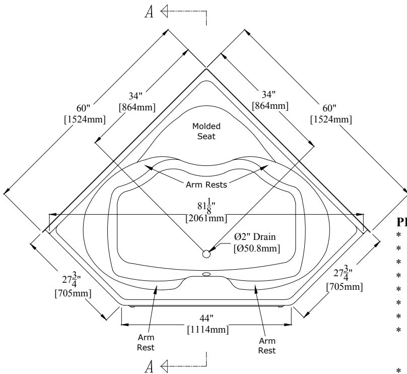
60" [1524mm] Corner Bathtub w/ Removable Access Panel, Molded Seat, & Molded Arm Rests
